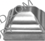
SC1 Sq. 1" 500pcs/Box 0.03 Lbs. SC114 Sq. 1-1/4" 400pcs/Box 0.046 Lbs. SC112 Sq. 1-1/2" 400pcs/Box 0.065 Lbs. SC2 Sq. 2" 400pcs/Box 0.1 Lbs.
